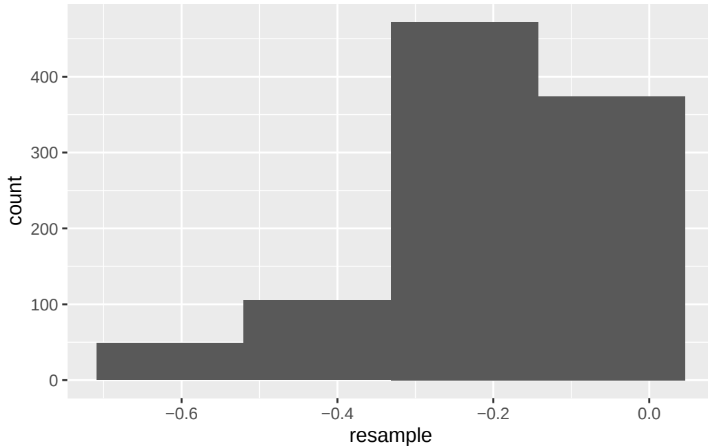
Figure 5: histogram of the farther resampling values
