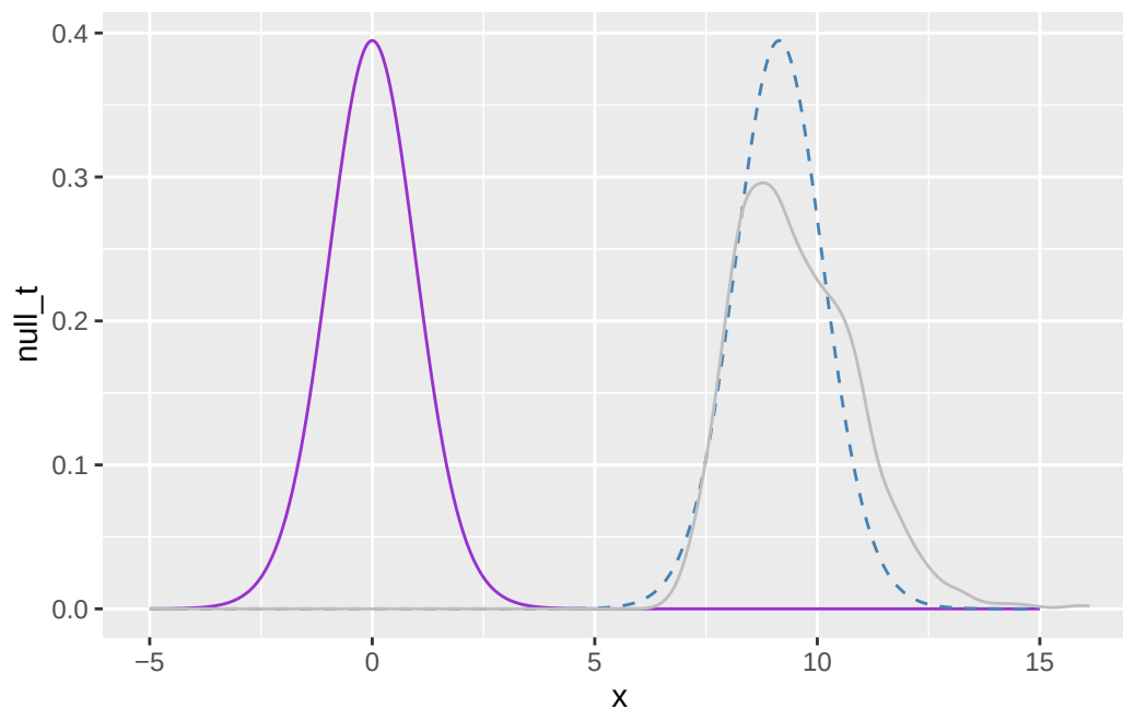
Figure 10: t-distributions for the differences
